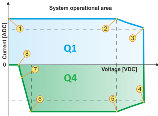
Q1 and Q4 range of device TC.DSS.32.400.815.S.
