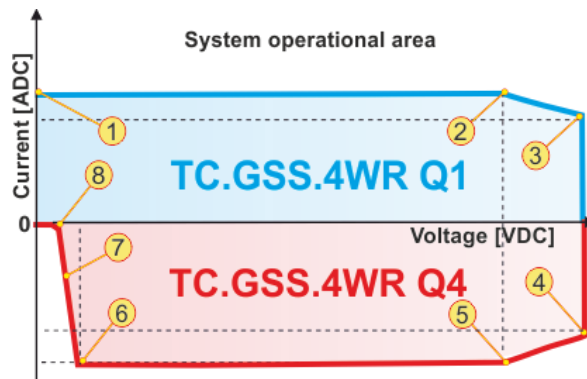
Q1 and Q4 range of device TC.GSS.20.65.4WR.S.
