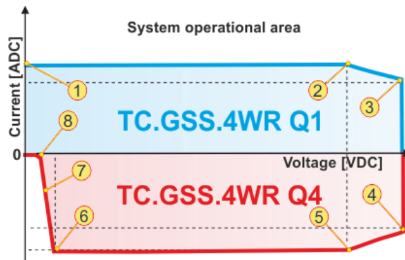
Q1 and Q4 range of device TC.GSS.32.500.4WR.S.
